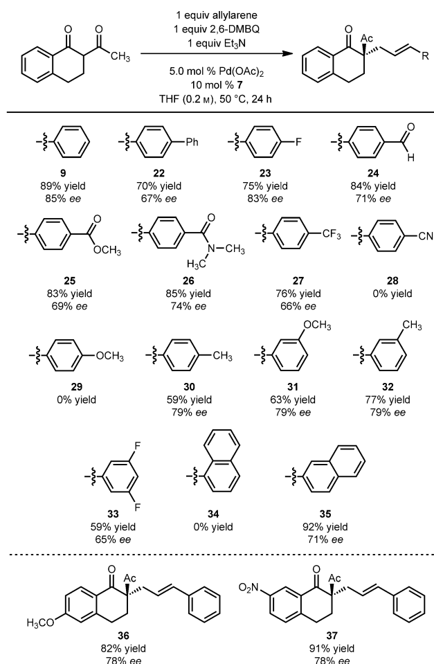
Scheme 4. Substrate scope of palladium-catalyzed enantioselective allylic alkylations through C–H alkylation. Catalyst added in two portions: 2.5 mol % Pd(OAc) 2 and 5 mol % 7 at the beginning of the reaction and 2.5 mol % Pd(OAc) 2 and 5 mol % 7 after 3 h; reactions performed on a 0.100 mmol scale. The absolute stereochemistry of the products was assigned by analogy to 9 , the configuration of which was determined to be S by a comparison of its optical rotation to that reported in a previous synthesis. [21] See the Supporting Information for details.
